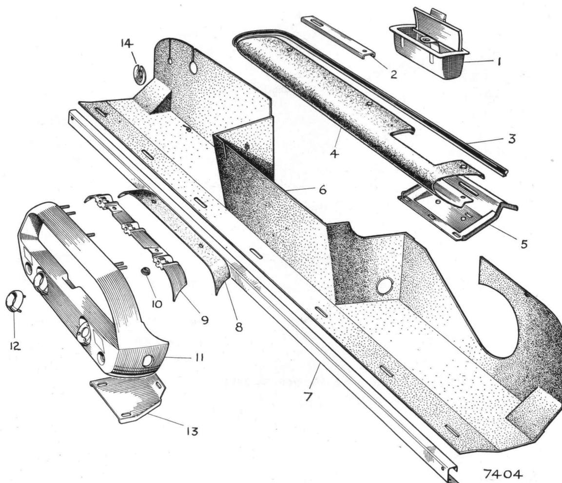
Fig. 13 Facia components
