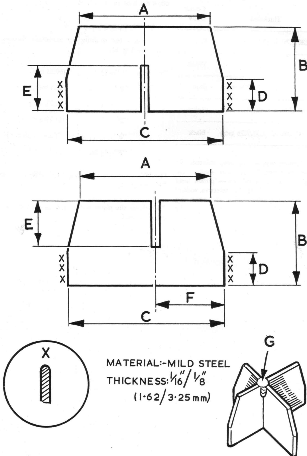
FIG. 67 TEMPLATE FOR ASSEMBLY FIXTURE
