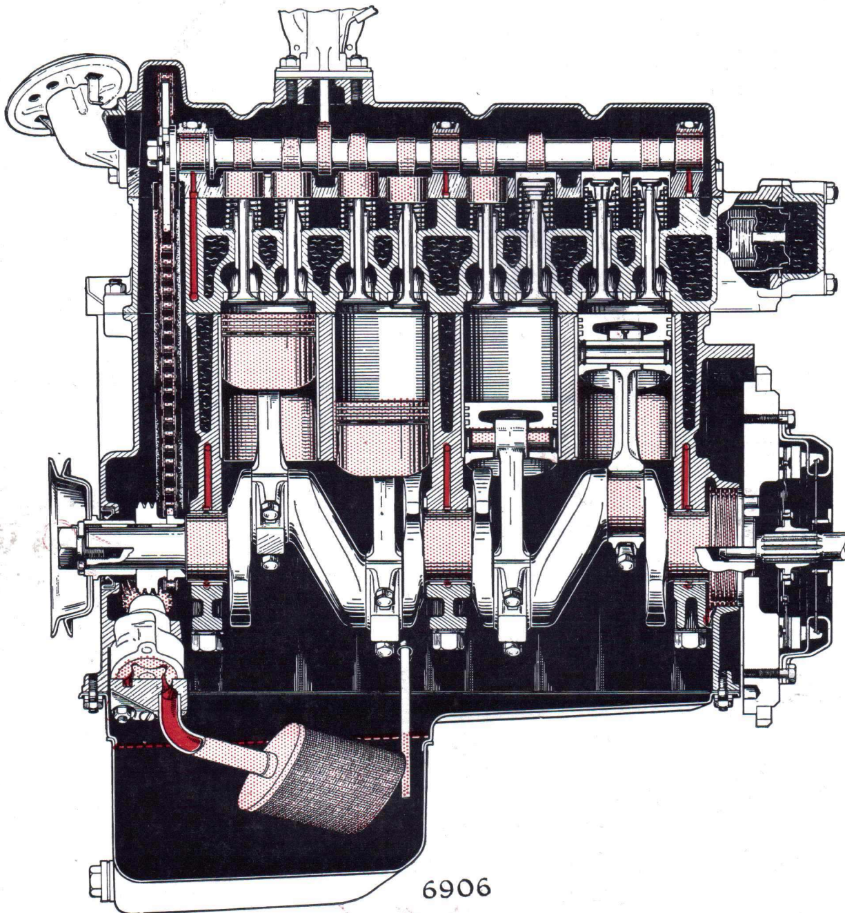
Fig. 1. Engine—longitudinal section
